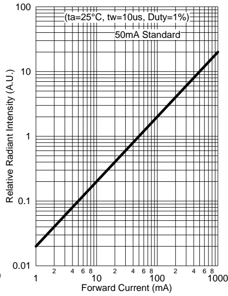
Relative Radiant Intensity - Forward Current
