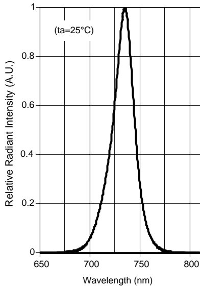
Peak Wavelength
