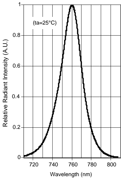
Peak Wavelength
