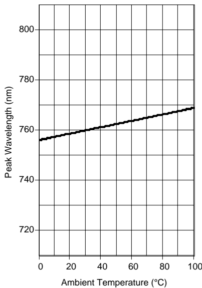
Peak Wavelength - Ambient Temperature
