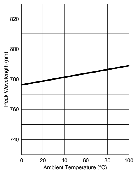
Peak Wavelength - Ambient Temperature
