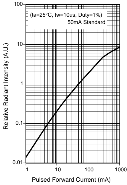
Relative Radiant Intensity - Pulsed Forward Current
