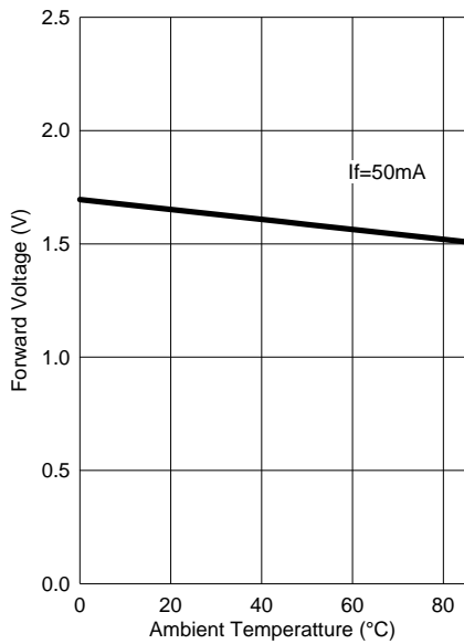
Forward Voltage - Ambient Temperature
