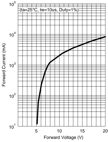
Forward Current - Forward Voltage
