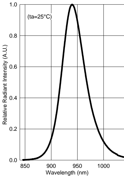
Peak Wavelength
