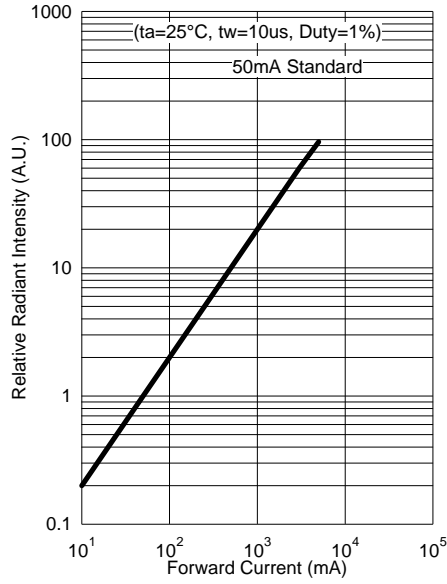
Relative Radiant Intensity - Forward Current
