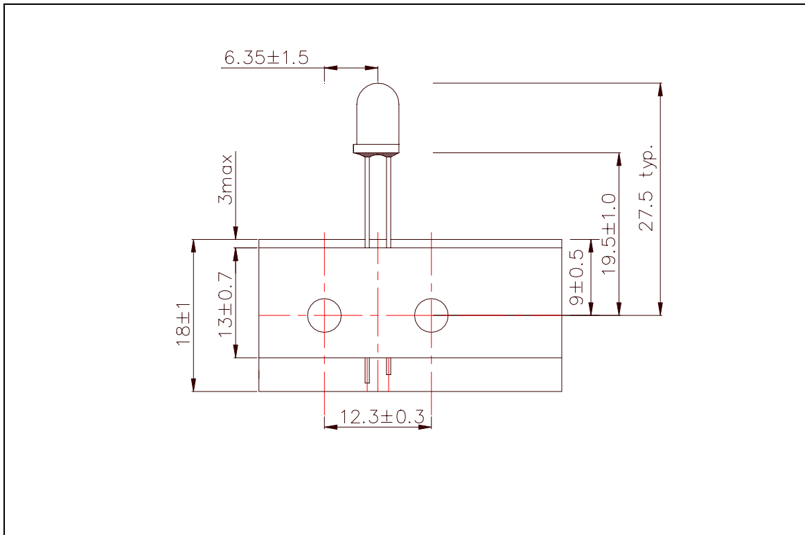
Taping dimension at 03 mold tape.
