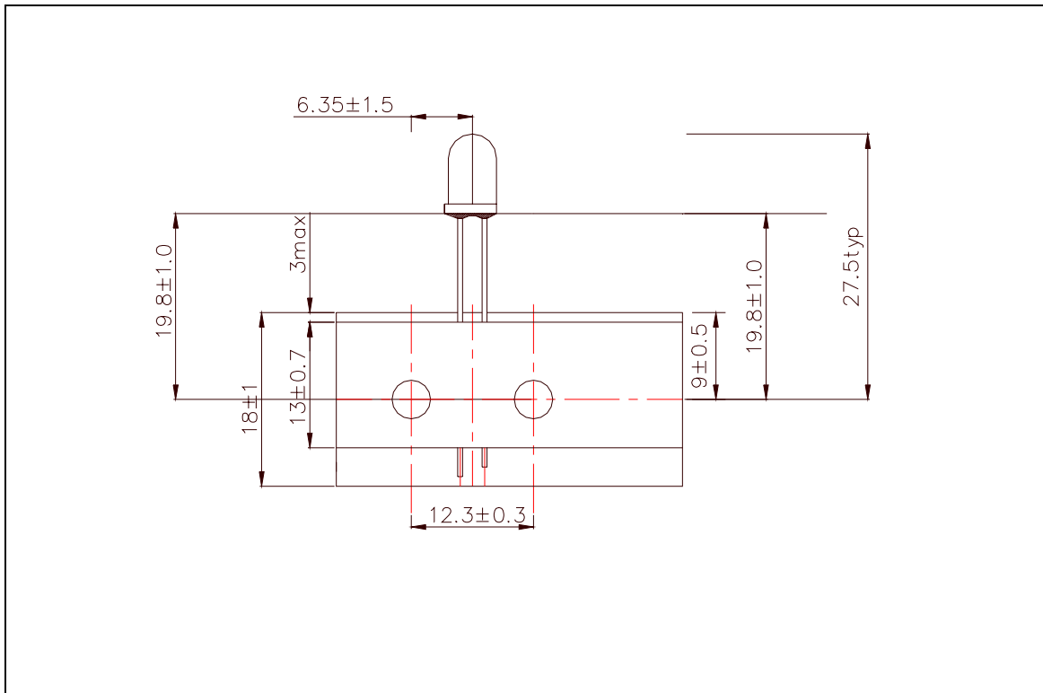
Taping dimension at 04 mold tape.
