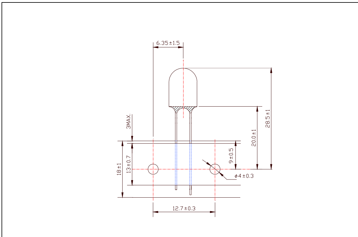
Taping dimension at 06 mold tape.
