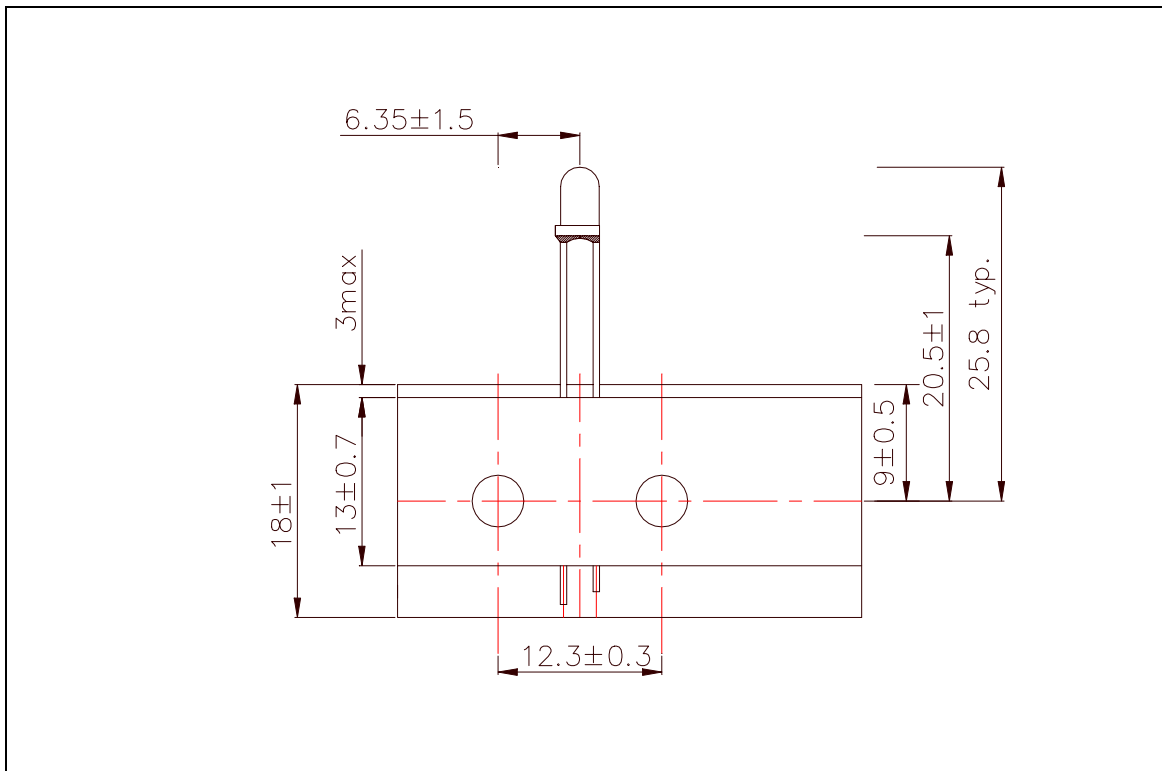
Taping dimension at 33 mold tape.
